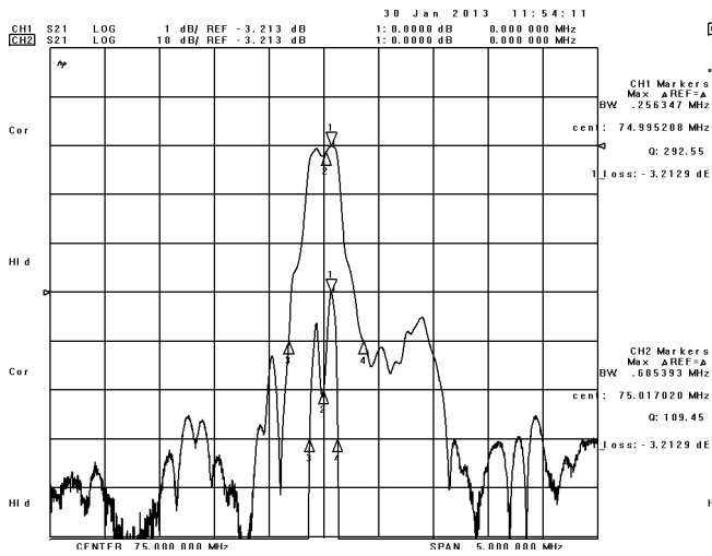
Frequency Response
