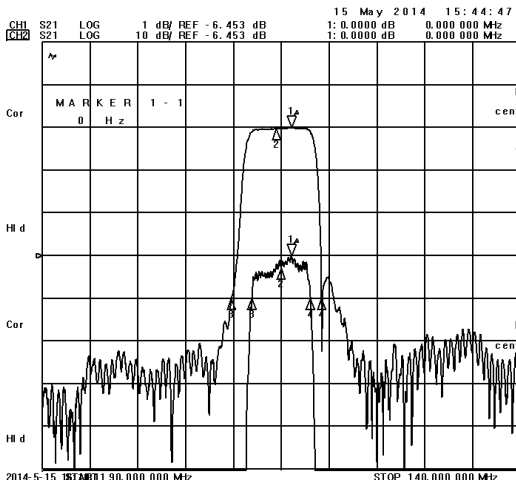
Frequency Response
