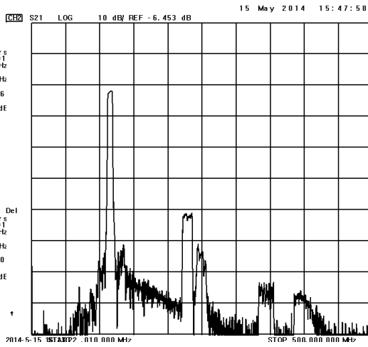
Frequency Response (wideband)
