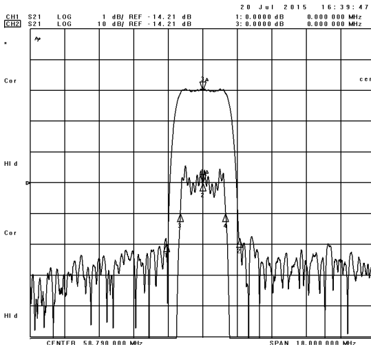
Frequency Response
