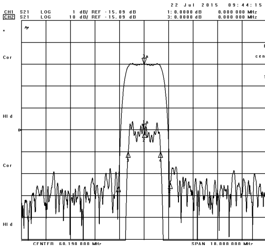
Frequency Response
