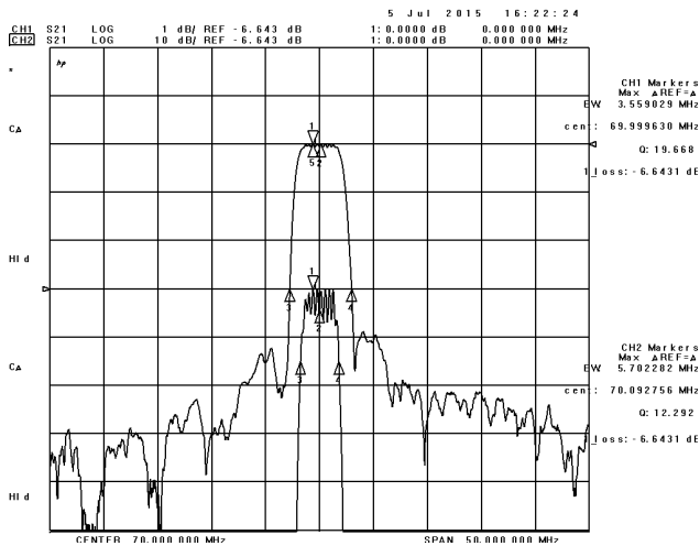
Frequency Response
